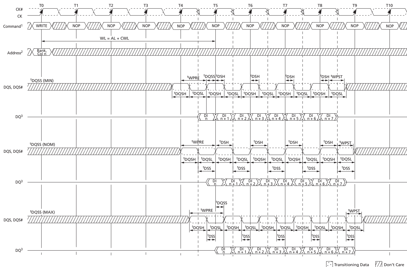
Figure 85: WRITE Burst
