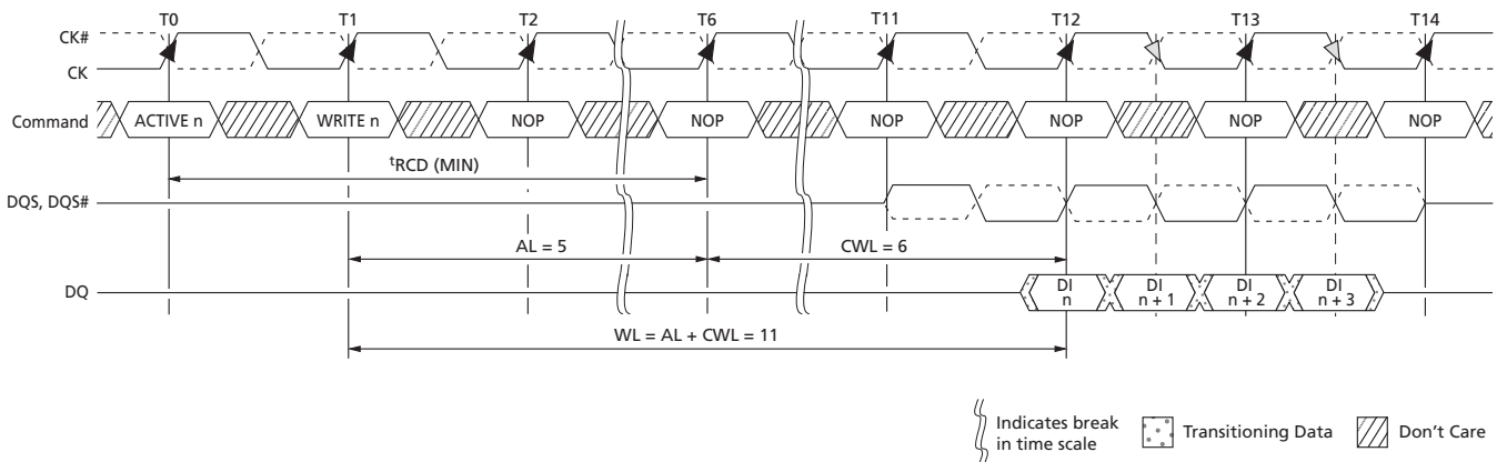
Figure 58: CAS Write Latency
