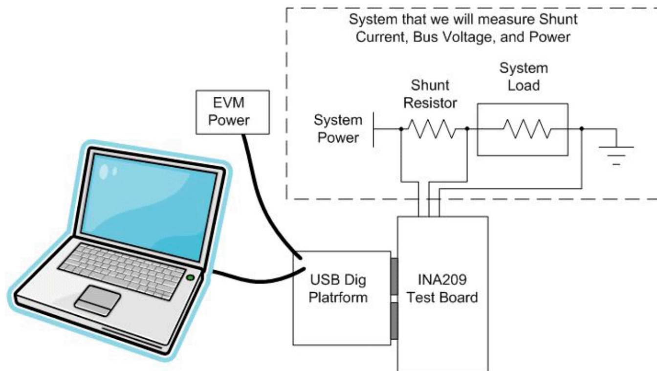
Figure 2. Hardware Setup for the INA209EVM
