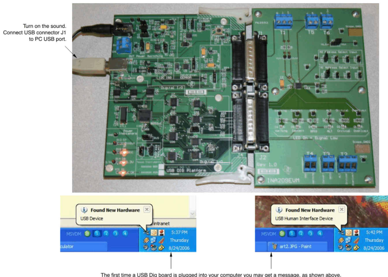
Figure 9. Connecting the USB Cable
