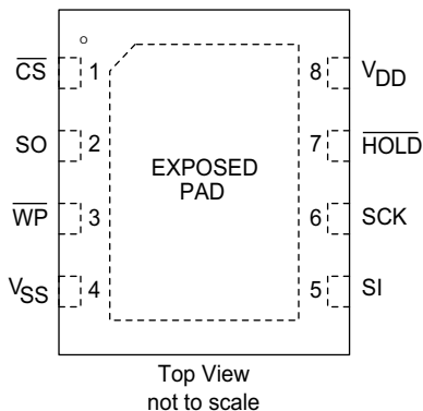
Figure 1. 8-pin DFN Pinout
