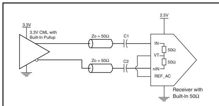
Figure 1E. IN/nIN Input with Built-In 50Ω Driven by a 3.3V CML Driver with Built-In Pullup
