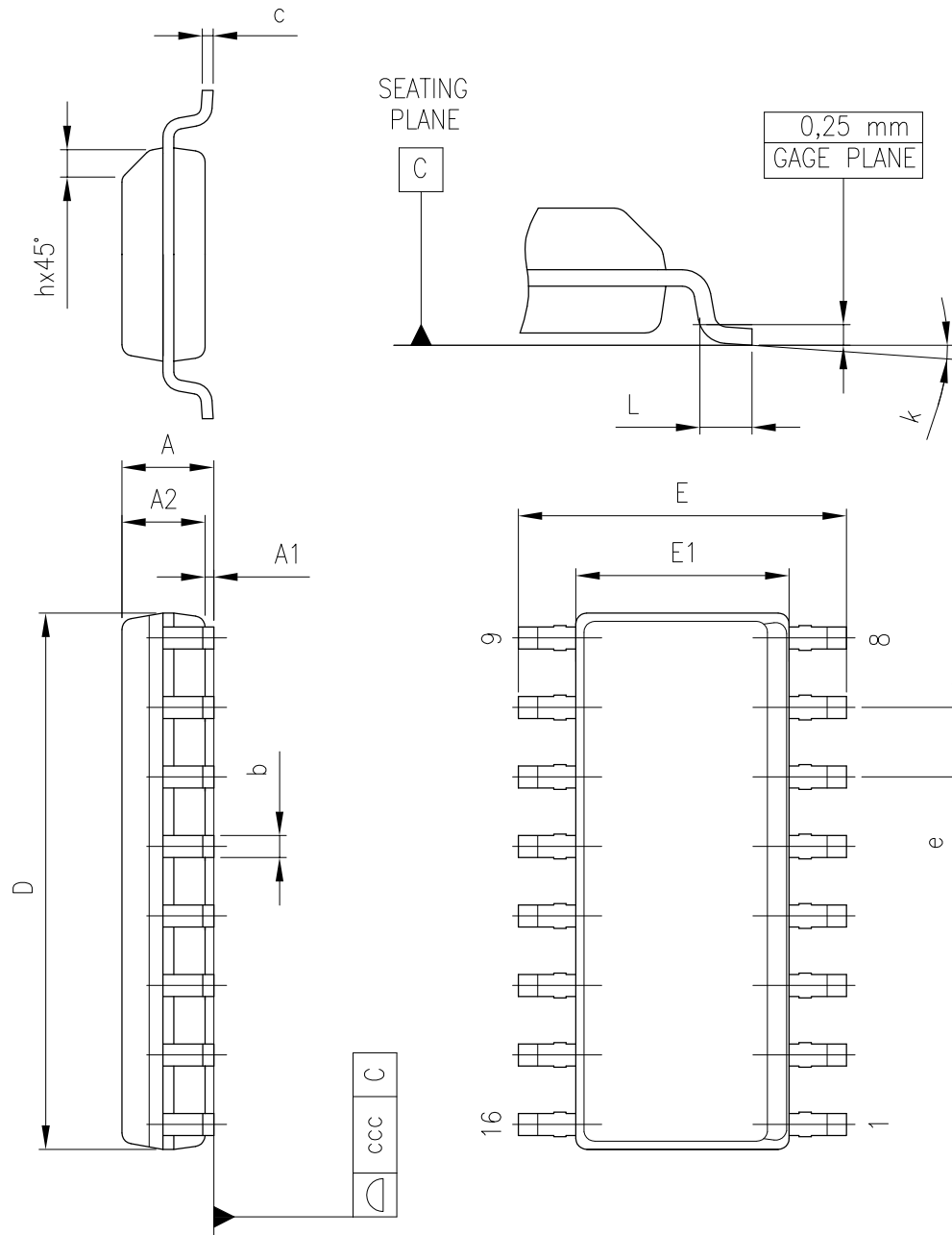
Figure 36. SO-16 narrow package dimensions
