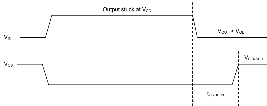
Figure 8. Openload off-state delay timing
