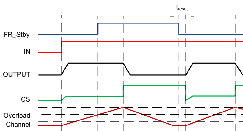
Figure 5. t_{reset} definition
