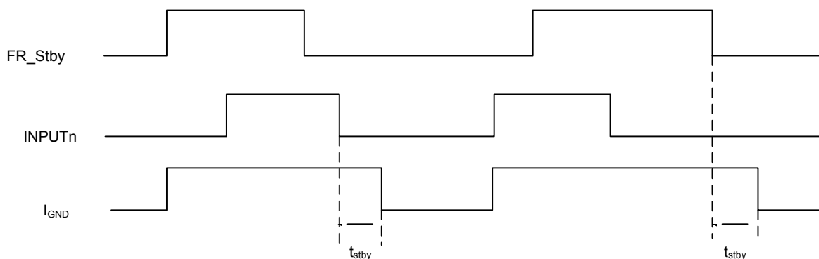
Figure 6. t_{stby} definition
