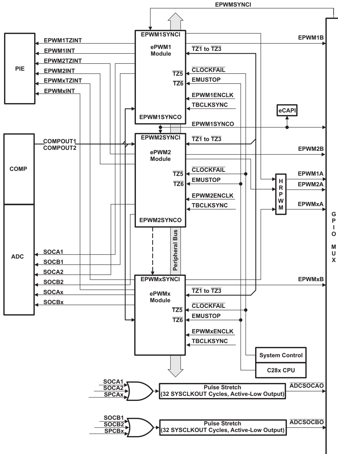
Figure 6-35. ePWM
