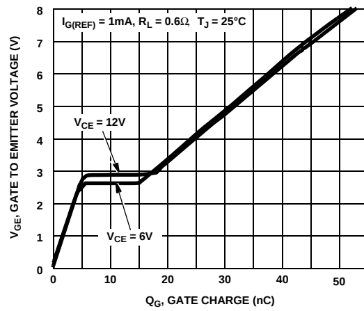
Figure 14. Gate Charge
