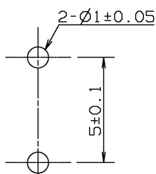
P.C.B.piercing plan
