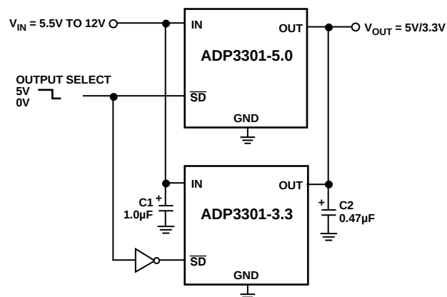
Figure 21. Crossover Switch
