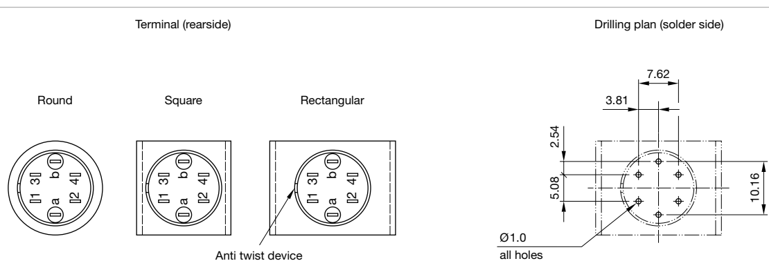
Component layout 3
