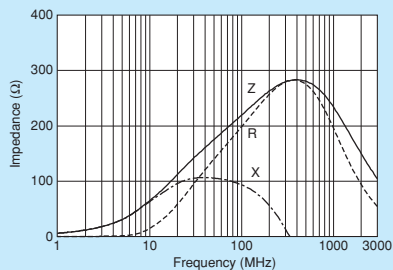
BLM15AX221SZ1
