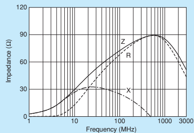
BLM18SG700TZ1
