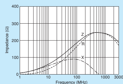
BLM18EG181SH1
