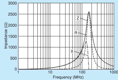
NFZ32BW6R8HZ11
