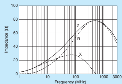
BLM21PG600SZ1/BLM21PG600SH1
