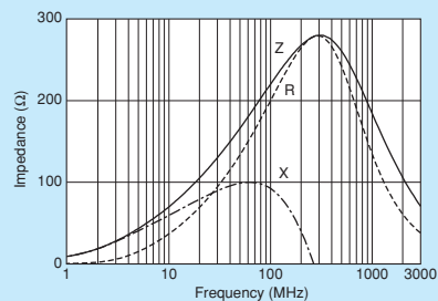
BLM18AG221SZ1/BLM18AG221SH1
