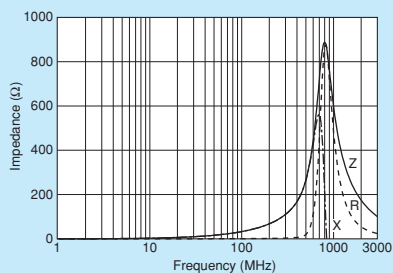
BLM15BA330SZ1
