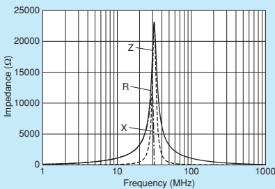
NFZ32BW101HZ11
