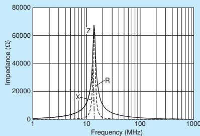
NFZ32BW621HZ10
