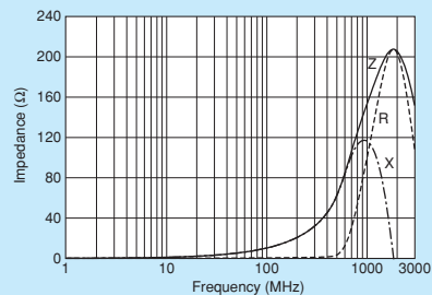
BLM15BA100SZ1
