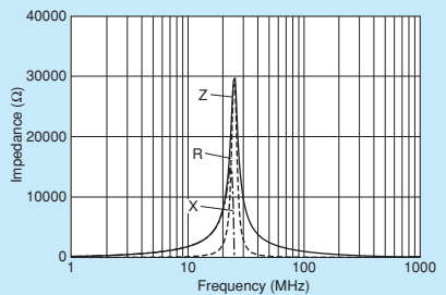
NFZ32BW151HZ11
