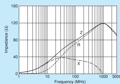
BLM03AG800SZ1
