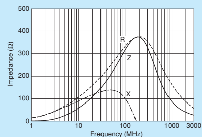
BLM21PG331SZ1/BLM21PG331SH1
