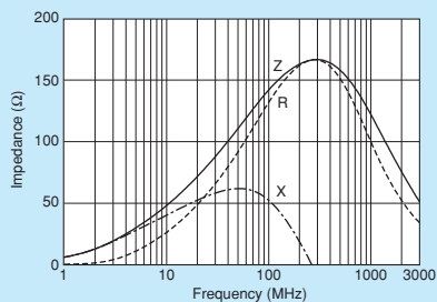
BLM21AG151SZ1/BLM21AG151SH1
