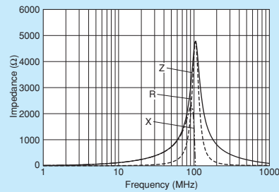
NFZ32BW120HZ11
