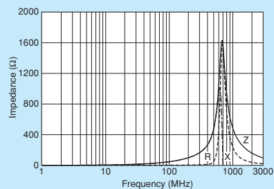
BLM15BA470SZ1
