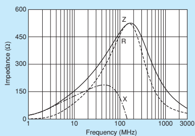
BLM21AG471SZ1/BLM21AG471SH1
