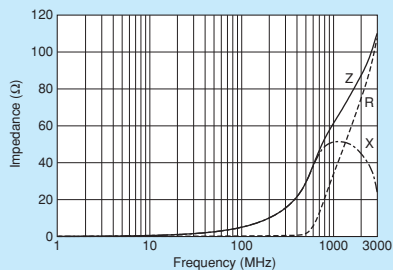
BLM15BA050SZ1
