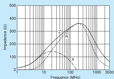
BLM18SG331TZ1
