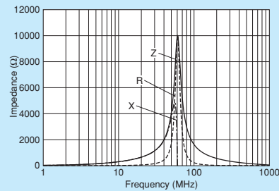
NFZ32BW310HZ11
