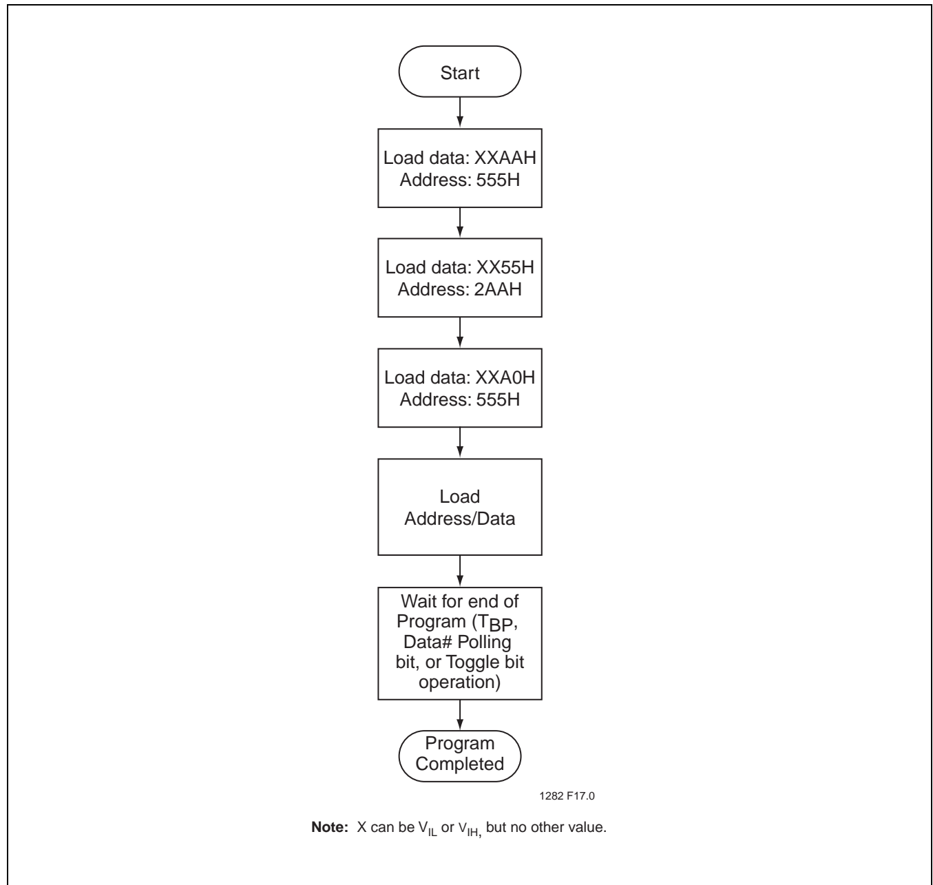
FIGURE 21: PROGRAM ALGORITHM
