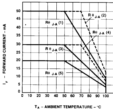
Figure 5. Maximum Forward dc Current vs. Ambient Temperature. Derating Based on T_J \text{ MAX} = 110^\circ\text{C} (Non-Resistor Lamps).
