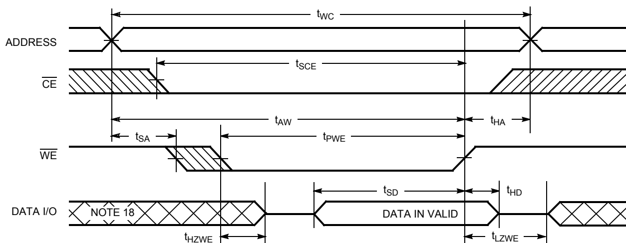
Figure 7. Write Cycle No. 3 ( \overline{\text{WE}} Controlled, \overline{\text{OE}} LOW) [3, 17, 19]
