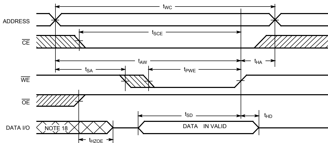
Figure 7. Write Cycle No. 3 ( \overline{\text{WE}} Controlled, \overline{\text{OE}} LOW) [3, 17, 19]
