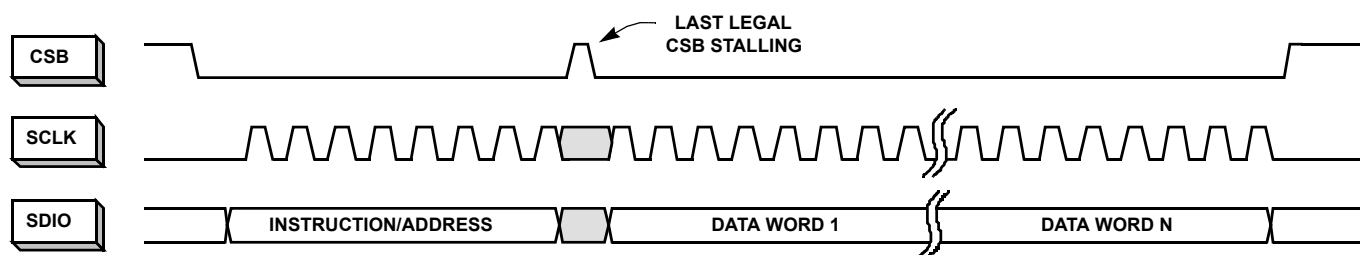
FIGURE 40. N-BYTE TRANSFER
