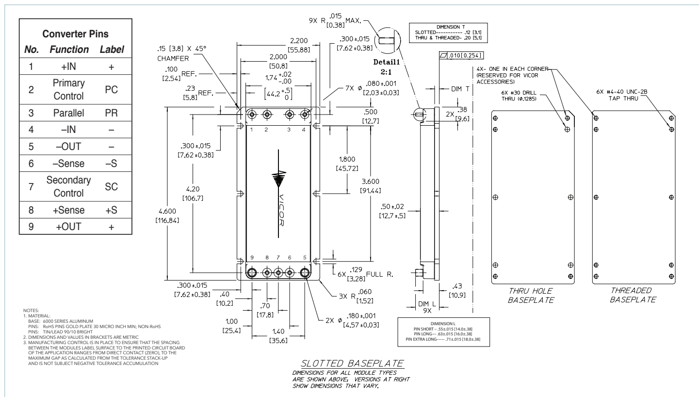
Figure 12 — Module outline
