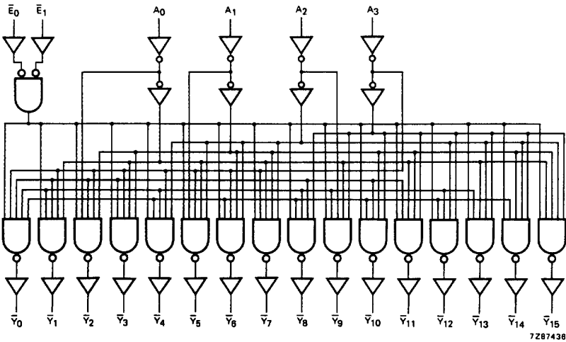
Fig.5 Logic diagram.
