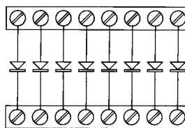
TYPE CIM/8W-D10
