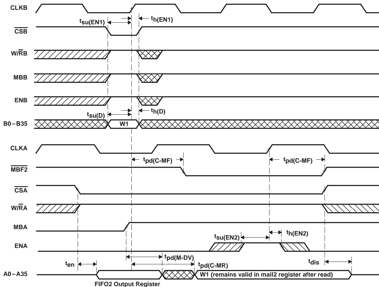
Figure 15. Timing for Mail2 Register and MBF2 Flag
