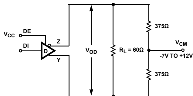
FIGURE 2B. V_{OD} WITH COMMON MODE LOAD
