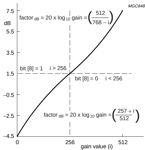
Fig.9 Amplifier curve.
