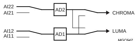
Fig.33 Mode 5 Y (automatic gain) + C (gain channel 2 fixed to GAI1 level).
