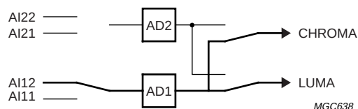
Fig.29 Mode 1; CVBS (automatic gain).
