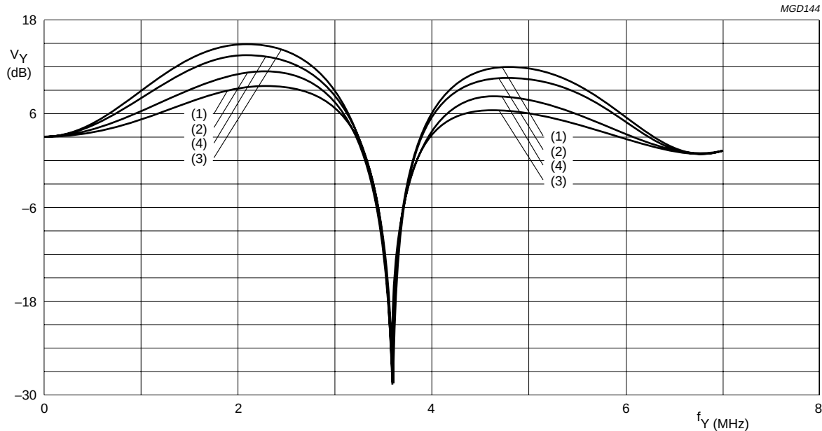
Fig.42 Luminance control SA 09H, 3.58 MHz Trap/CVBS mode, prefilter on and different aperture band-pass centre frequencies.
