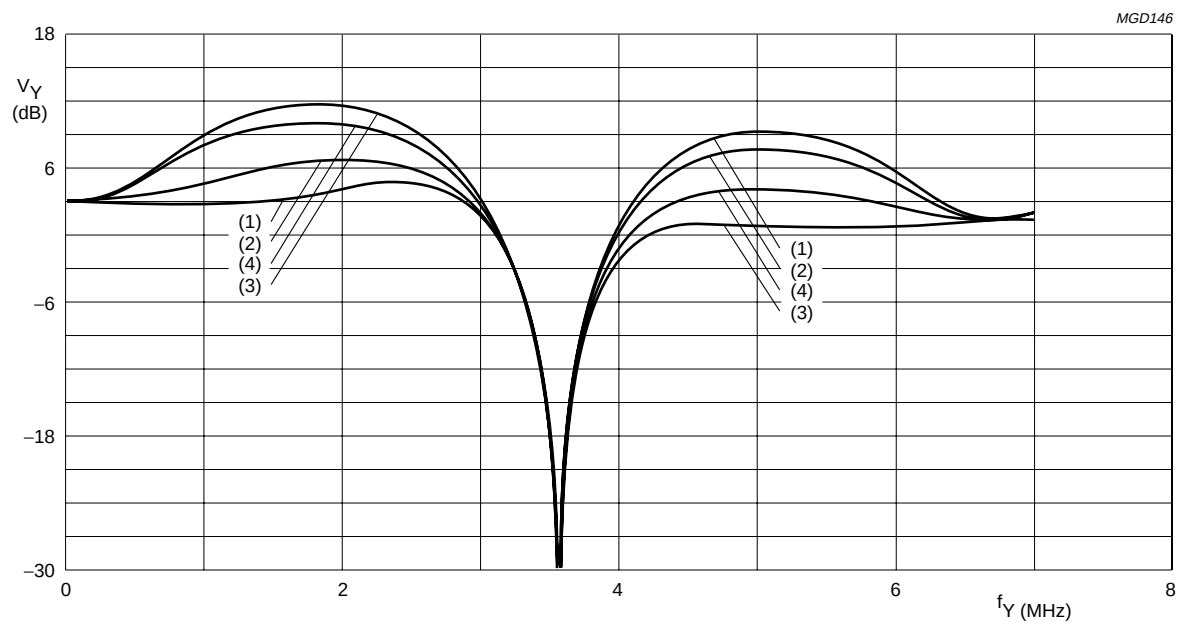
Fig.44 Luminance control SA 09H, 3.58 MHz Trap/CVBS mode, prefilter off and different aperture band-pass centre frequencies.
