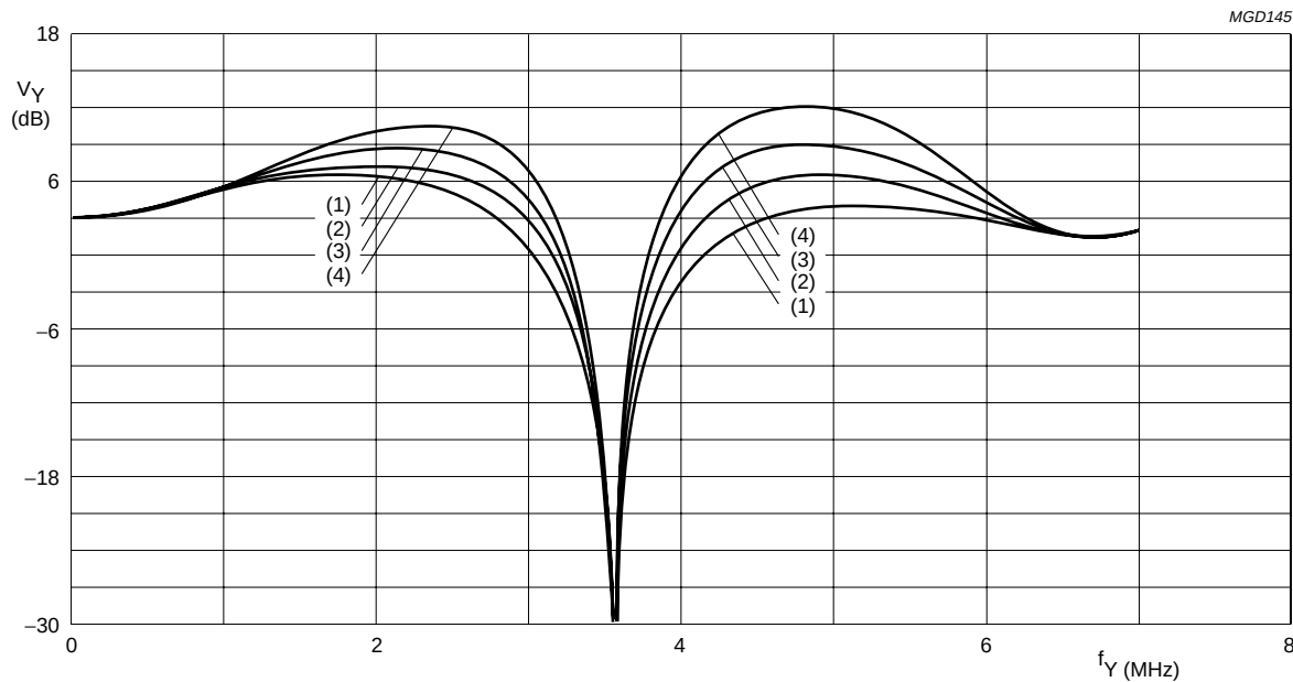
Fig.43 Luminance control SA 09H, 3.58 MHz Trap/CVBS mode, prefilter on and different aperture factors.
