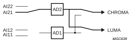
Fig.30 Mode 2; CVBS (automatic gain).
