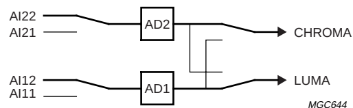
Fig.35 Mode 7 Y (automatic gain) + C (gain channel 2 adapted to Y gain).
