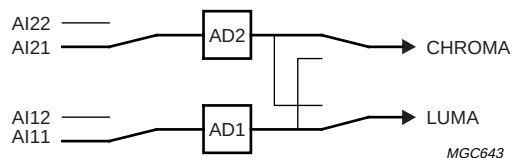
Fig.34 Mode 6 Y (automatic gain) + C (gain channel 2 adapted to Y gain).
