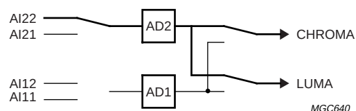
Fig.31 Mode 3; CVBS (automatic gain).
