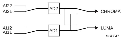
Fig.32 Mode 4 Y (automatic gain) + C (gain channel 2 fixed to GAI1 level).
