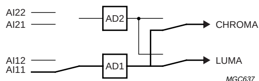
Fig.28 Mode 0; CVBS (automatic gain).
