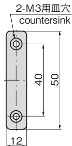
[C-74用受け金具] base plate
