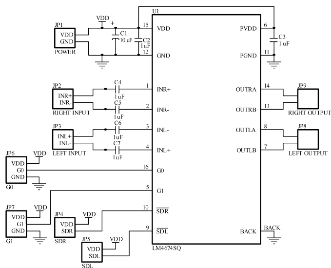
Figure 8-11. LM4674SQ Demo Board Schematic
