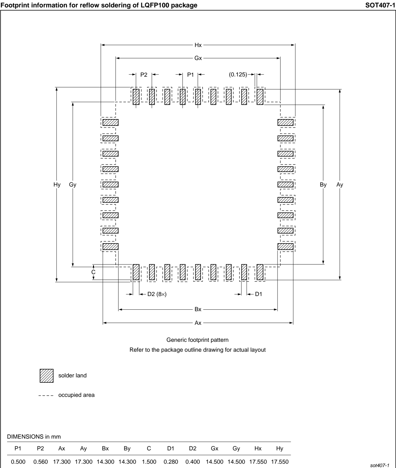
Fig 55. Reflow soldering for the LQFP100 package
