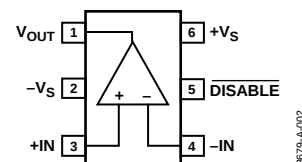
Figure 2. SC70-6 (KS)
