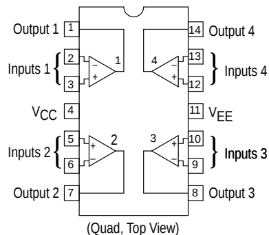
D SUFFIX PLASTIC PACKAGE CASE 751A (SO-14)
