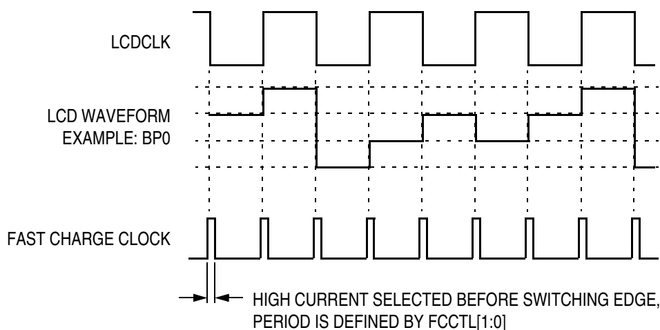
Figure 17-4. Fast Charge Timing
