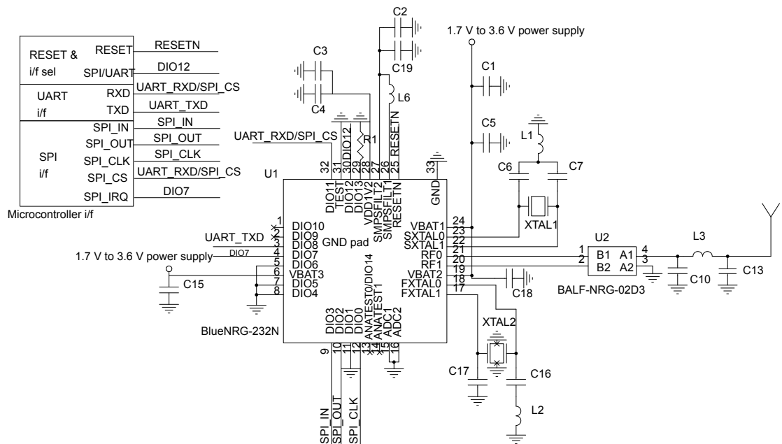
Figure 13. Application circuit: active DC-DC converter VFQFPN32 package with BALF-NRG-02D3 balun
