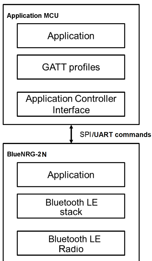
Figure 1. BlueNRG-2N network processor RF software layers
