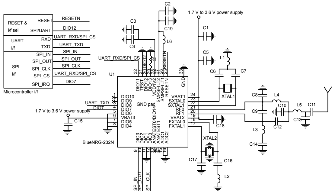
Figure 10. Application circuit: non-active DC-DC converter VFQFPN32 package
