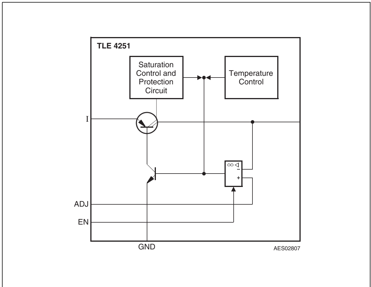
Figure 2 Block Diagram
