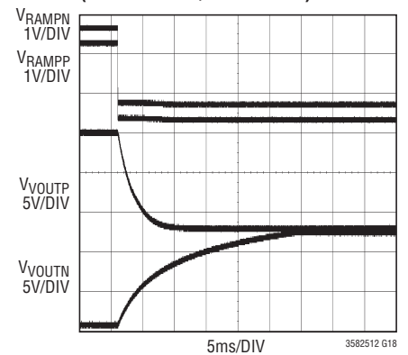
Power-Down Discharge Waveforms (PUSEQ = 11, PDDIS = 1)
