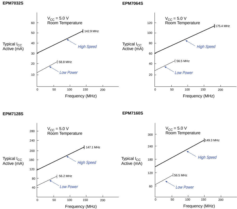
Figure 15. I_{CC} vs. Frequency for MAX 7000S Devices (Part 1 of 2)
