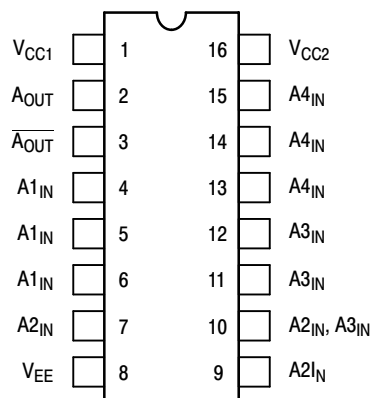
Figure 2. Pin Assignment
