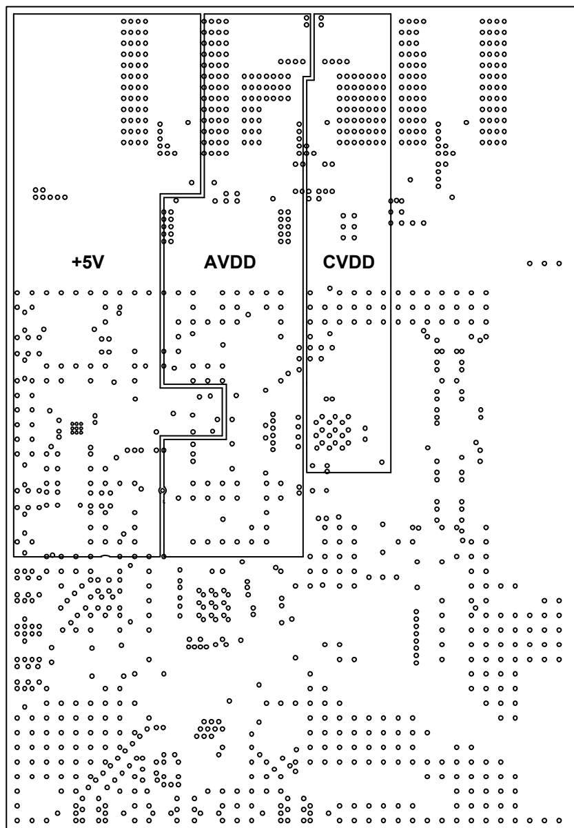
Figure 22. Power 1: Layer 3
