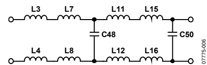
Figure 6. Fourth Order Filter
