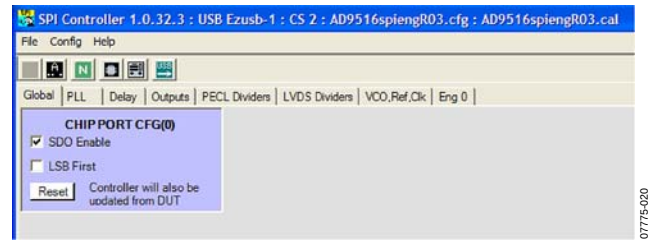
Figure 11. AD9516 Configuration
