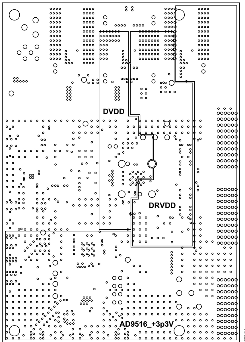
Figure 23. Power 2: Layer 4
