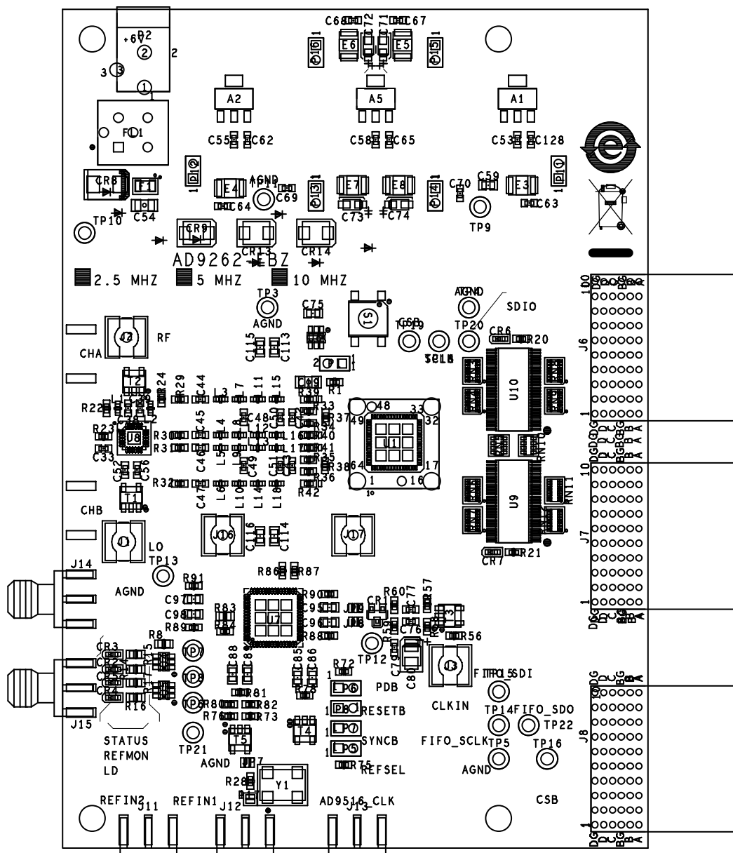
Figure 20. Top Silk
