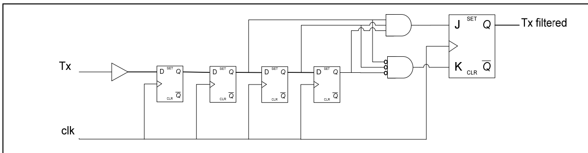
Figure 15-1: Noise Filter
