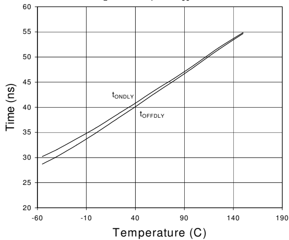
Propagation Delay Times vs. Temperature C_L = 1000pF V_{CC} = 18V
