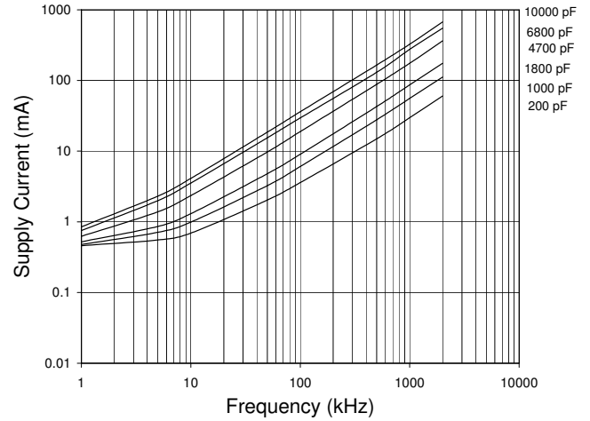
Supply Current vs. Frequency V_{CC} = 35V
