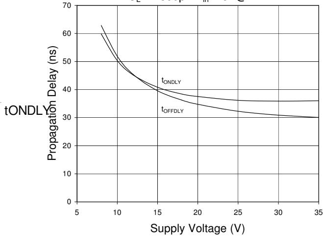
Propagation Delay vs. Supply Voltage C_L = 1800pF V_{in} = 5V@1kHz
