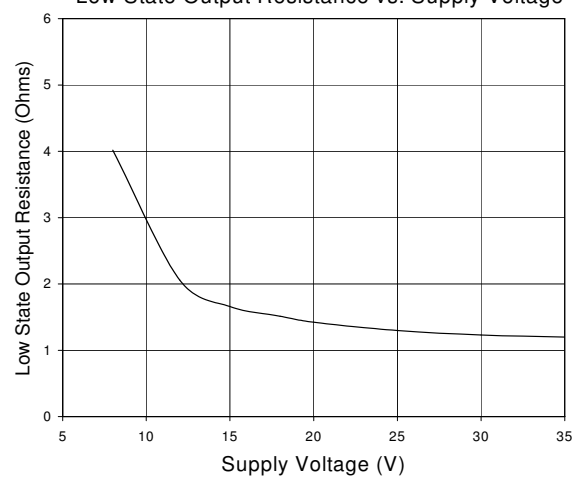
Fig. 22 Low State Output Resistance vs. Supply Voltage
