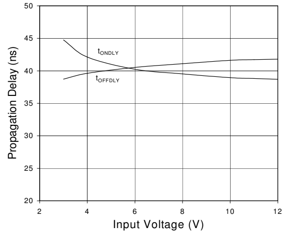
Propagation Delay vs. Input Voltage C_L = 1800pF V_{CC} = 15V
