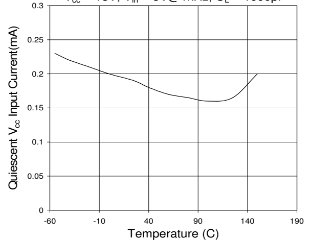
Quiescent Supply Current vs. Temperature V_{CC} = 18V , V_{in} = 5V@1kHz , C_L = 1000pF
