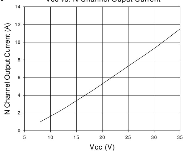
Fig. 24 Vcc vs. N Channel Output Current
