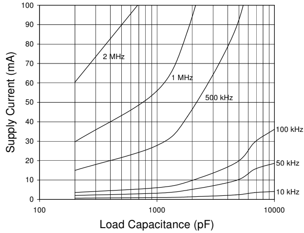
Supply Current vs. Load Capacitance V_{CC} = 35V
