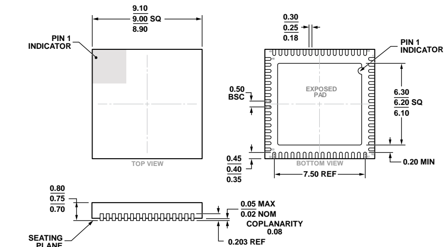
Figure 118. 64-Lead Lead Frame Chip Scale Package [LFCSP] 9 mm × 9 mm Body and 0.75 mm Package Height (CP-64-17)
