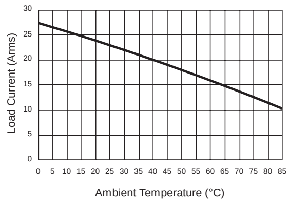
Figure 4a — DRD48X20
