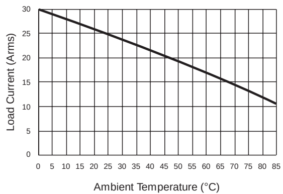
Figure 4b — DRD48D25
