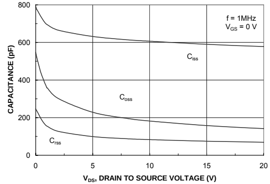
Figure 19. Capacitance Characteristics.
