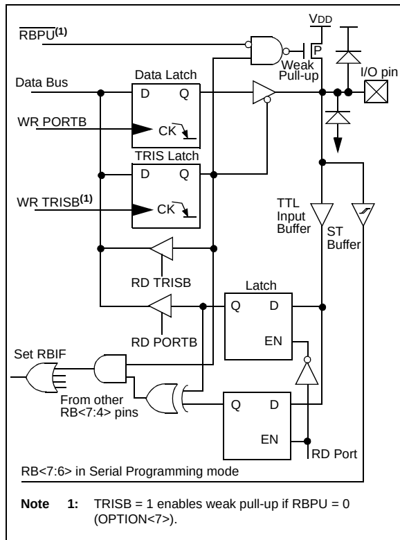
FIGURE 4-5: BLOCK DIAGRAM OF RB<7:4> PINS
