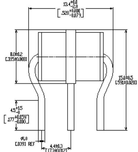
Axial Leaded (GTCA38-XXXM-R10)
