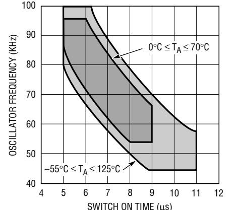
Minimum/Maximum Frequency vs ON Time
