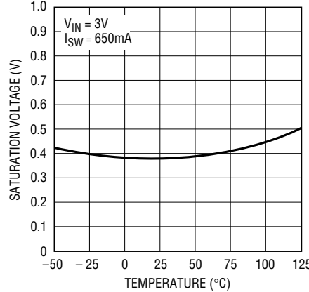
Saturation Voltage Step-Up Mode
