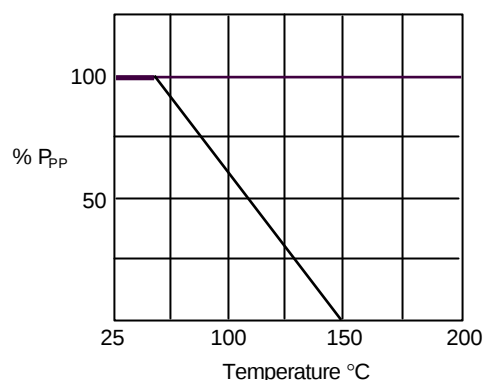
Figure 4 - Derating Curve
