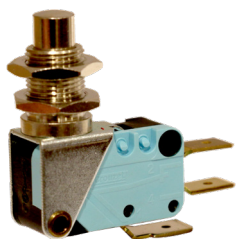
Telescopic plunger and adjustable fixing . 4mm overtravel. Metal version for heavy duty (SP9603)
