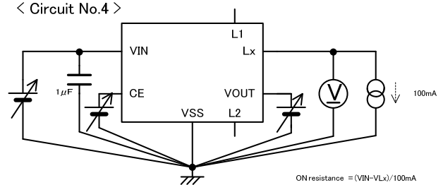
< Circuit No.4 >
