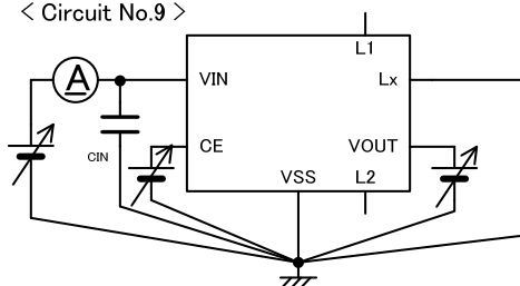
< Circuit No.9 >
