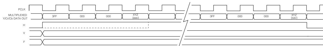
H:V:F TIMING - SD 10-BIT INPUT MODE
