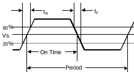
Figure 7. Output Waveform
