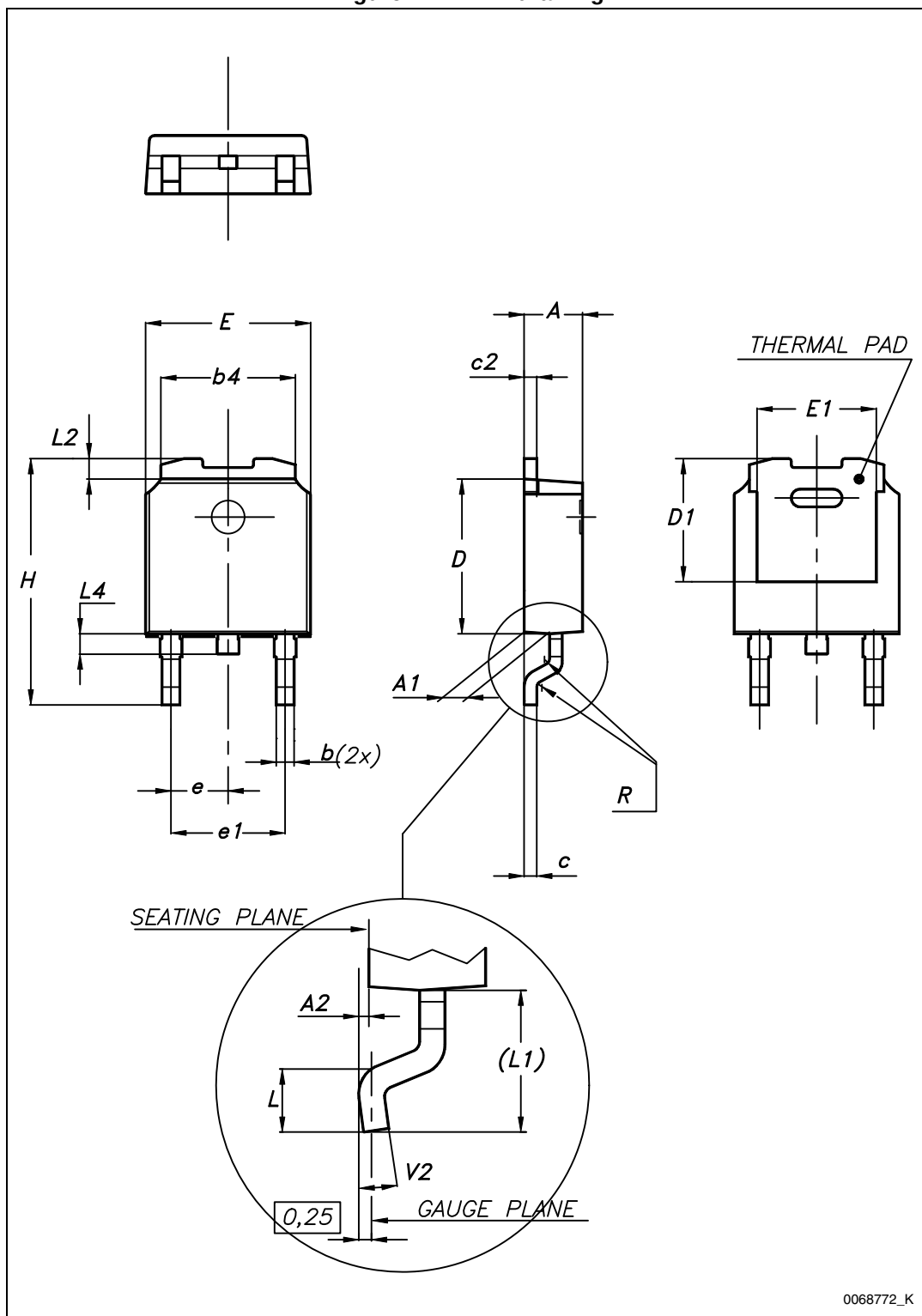
Figure 21. DPAK drawing
