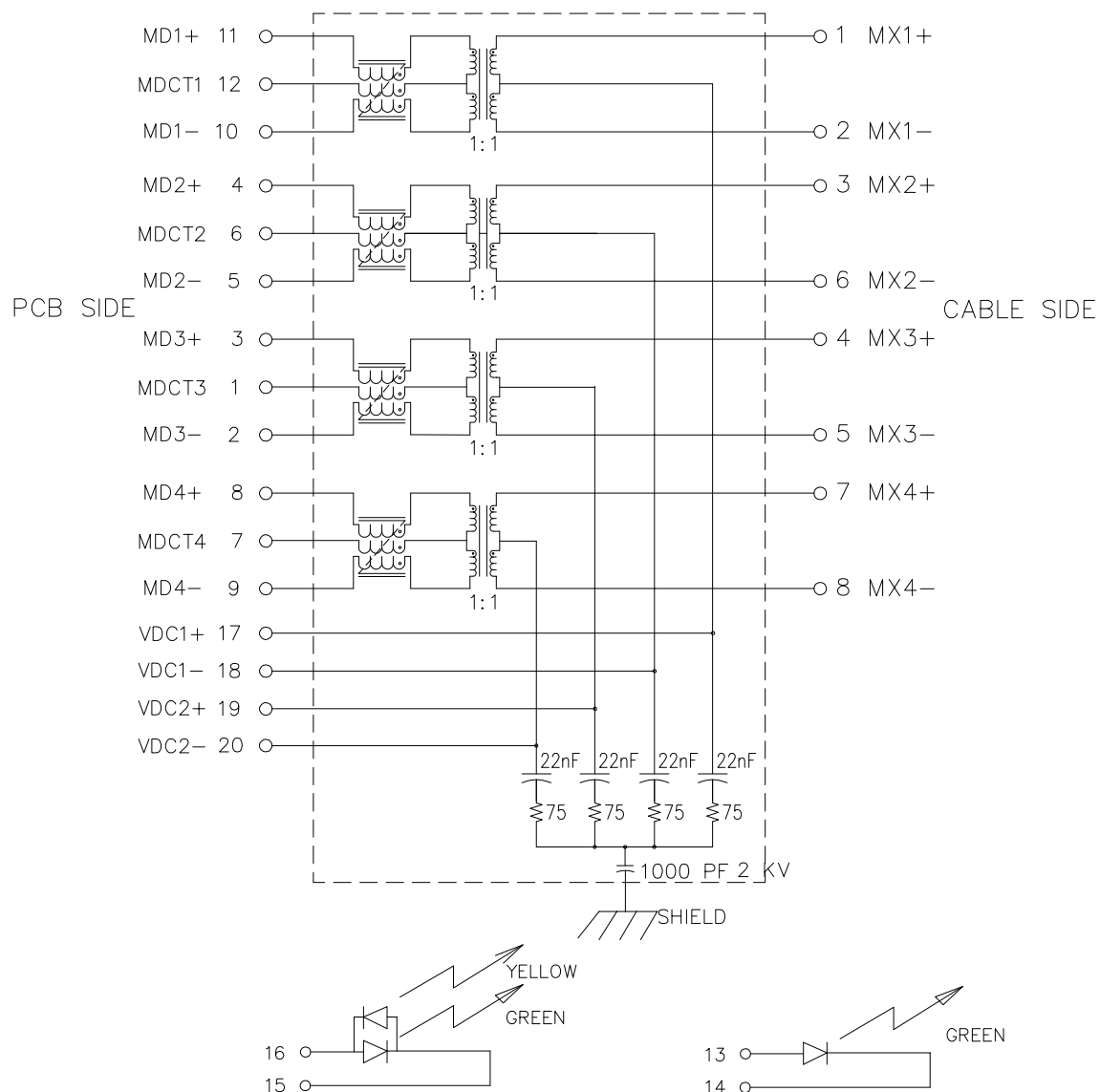
SCHEMATIC
