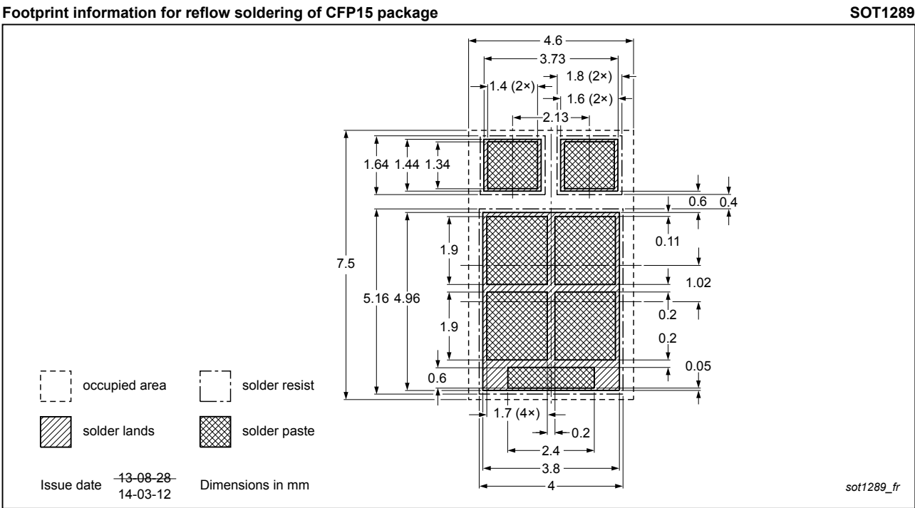
Fig. 18. Reflow soldering footprint for CFP15 (SOT1289)
