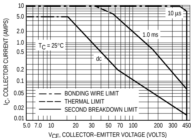
Figure 16. Maximum Rated Forward Bias Safe Operating Area (MJE16002 and MJE16004)
